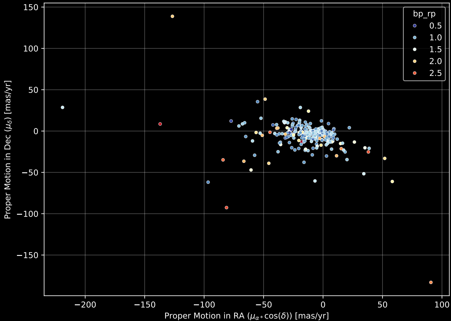
APOGEE DR17 Field: [M68] Proper Motion Diagram (n= 271)
