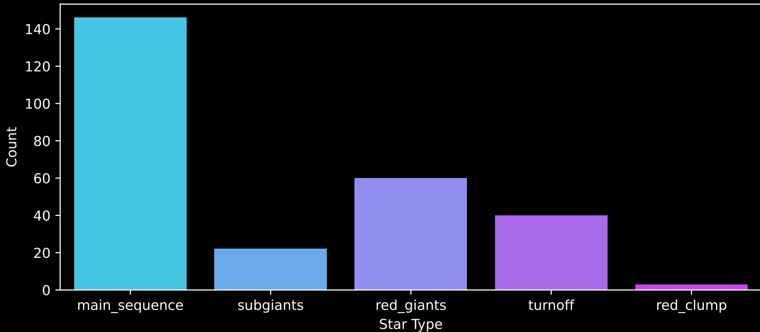
APOGEE DR17 Field: [M68] Count plot of Star Type
