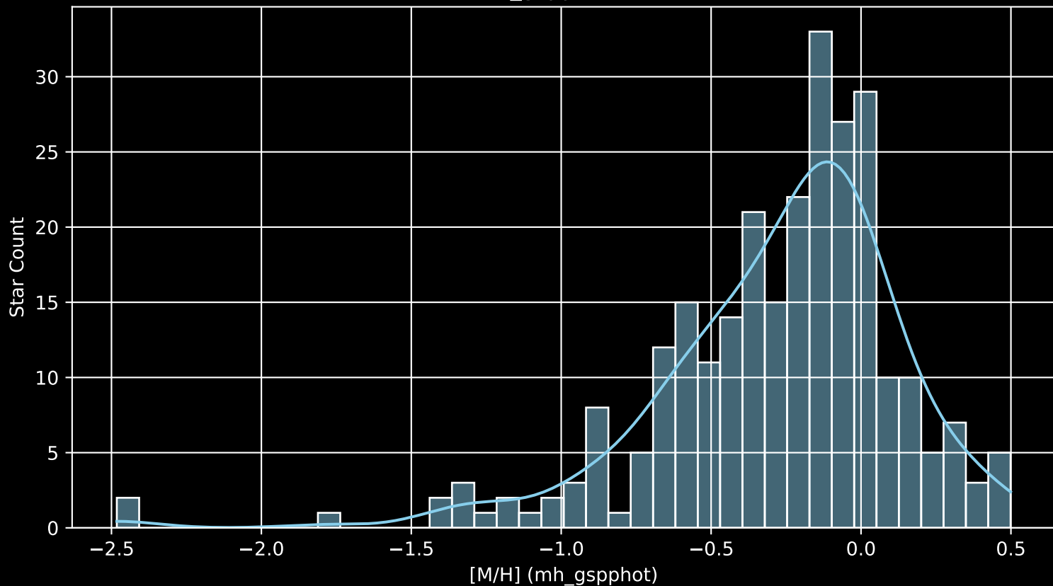
APOGEE DR17 Field: [M68 [M/H] (mh_gspphot) (n= 270)
