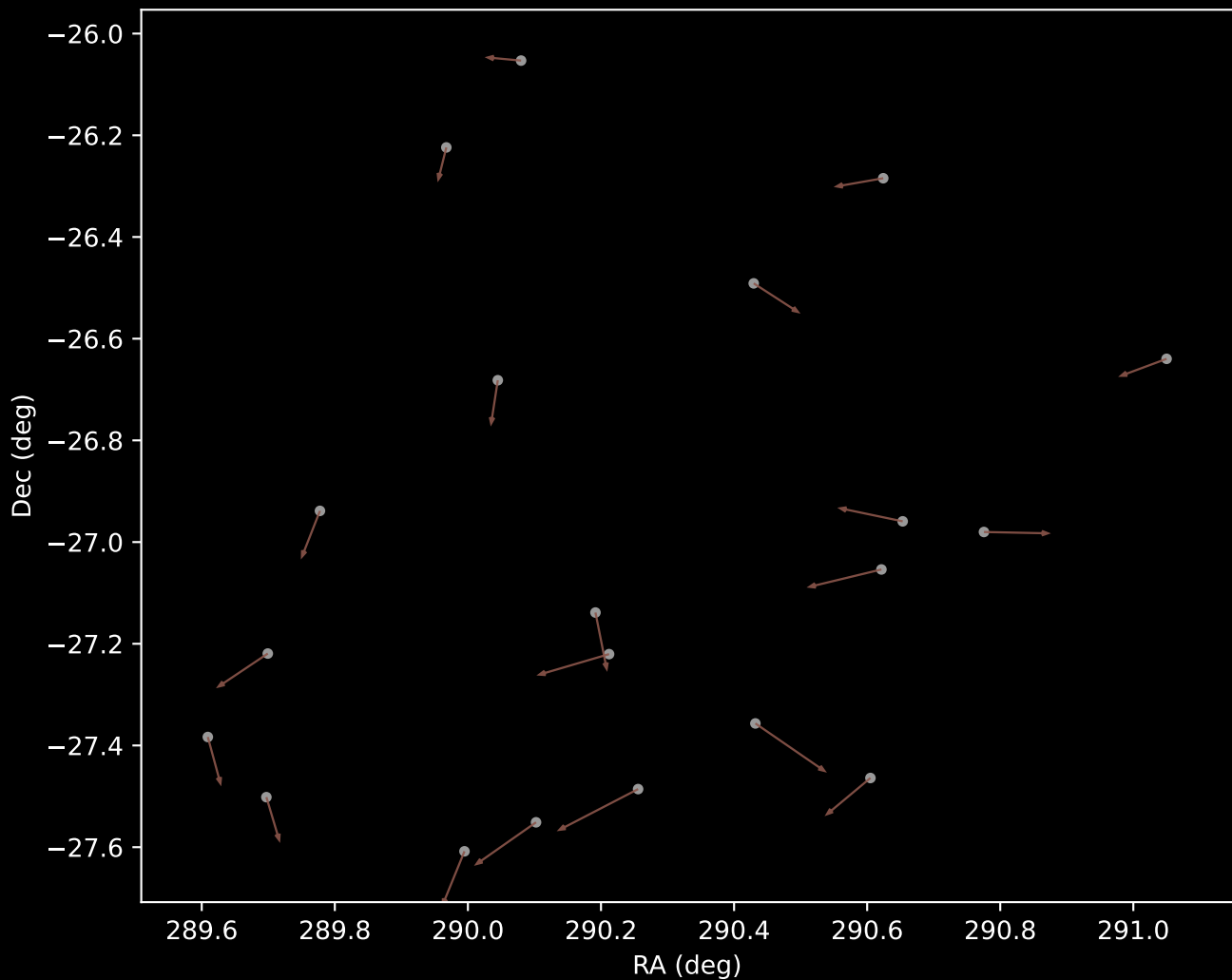
APOGEE DR17 Cluster 10 Proper Motion Vectors (n=20)
