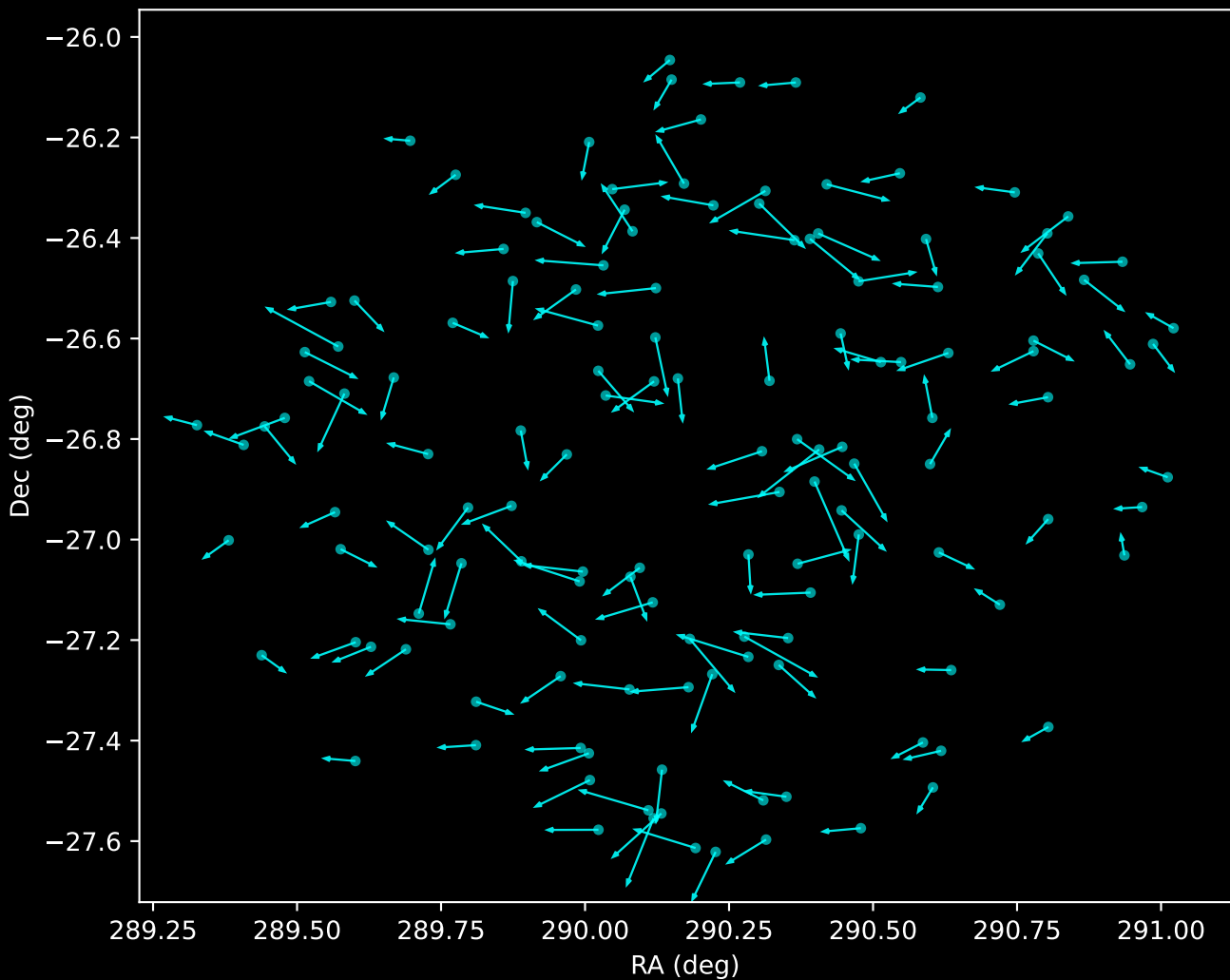
APOGEE DR17 Noise Stream Proper Motion Vectors (n=140)
