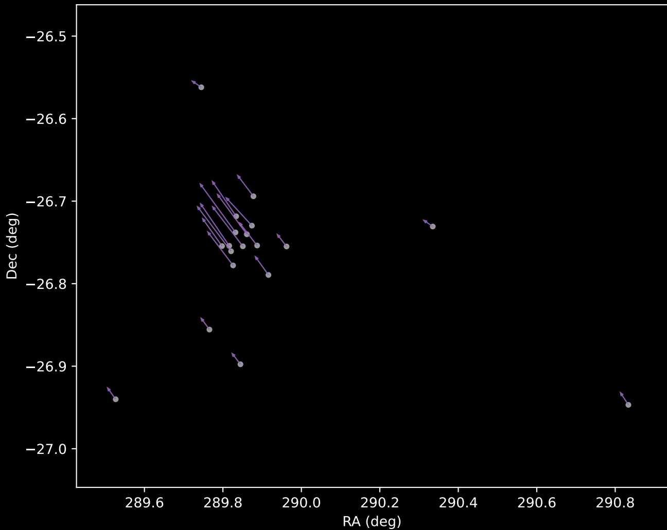
APOGEE DR17 Cluster 8 Proper Motion Vectors (n=19)
