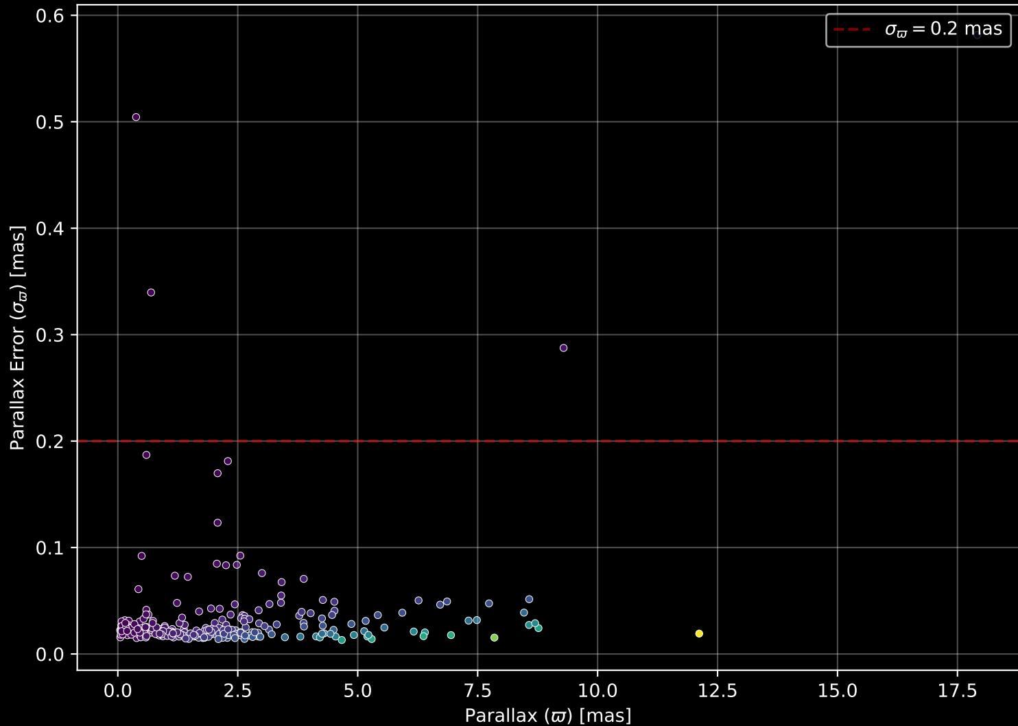
APOGEE DR17 Field: [M68] Parallax Quality (n= 271)
