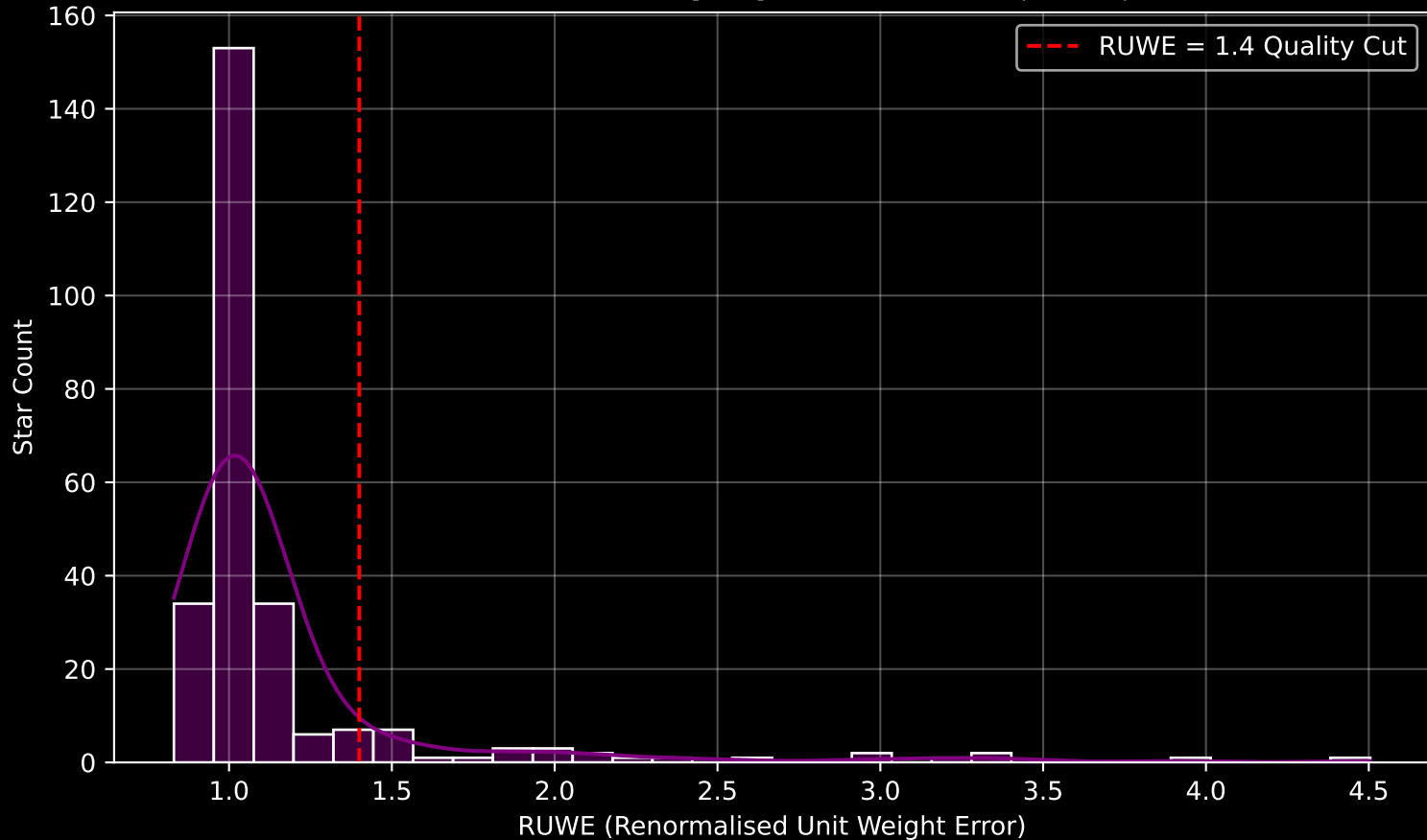
GAPOGEE DR17 Field [M68] RUWE Distribution (n= 261)
